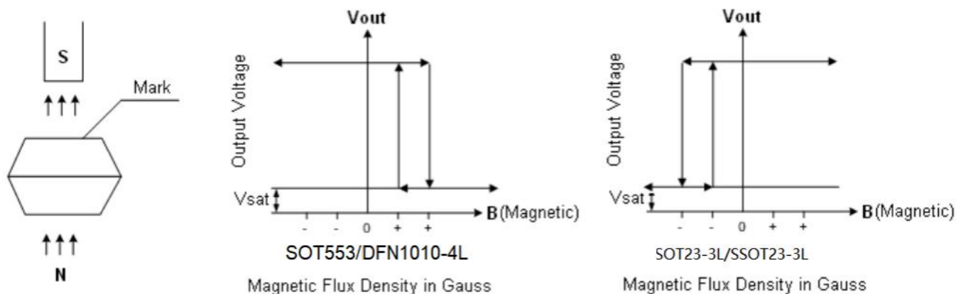
Fig 4, Magnetic Operation Characteristic of AS1918-L
