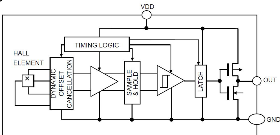
Figure 3, Block Diagram of AS1918-L
